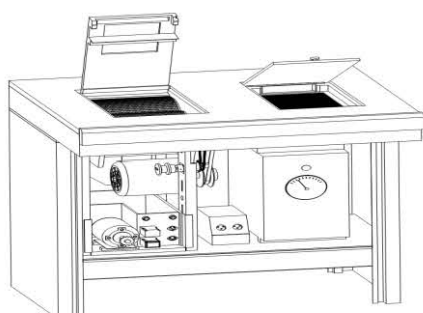
Fig. 2.5 Schematic diagram of the lint opener
