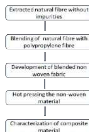
Fig. 2.43 Banana fibre based non-woven composite
