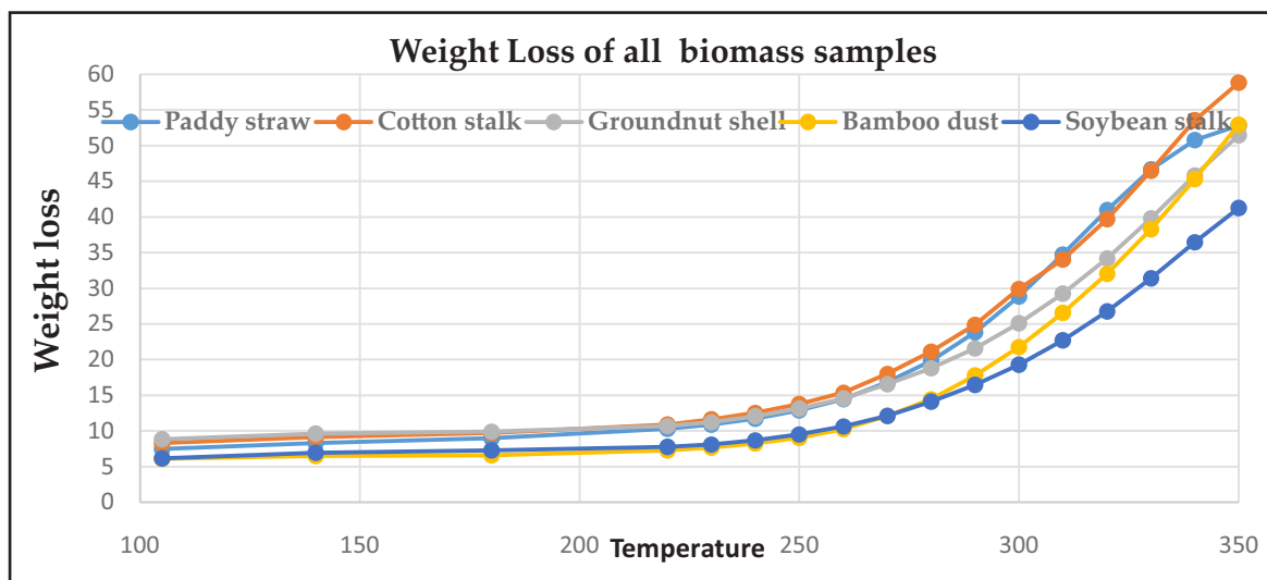
Fig 2.50 TGA pattern of various biomass samples
