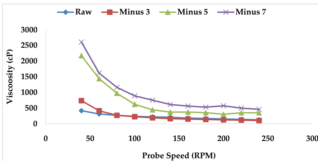
Fig. 2.24 : Variation in the viscosity of nano sulphur suspension with particle size reduction
