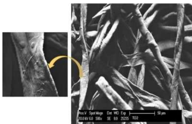
Fig. 2.33 Surface morphology of TEMPO-oxidized cotton fibres
