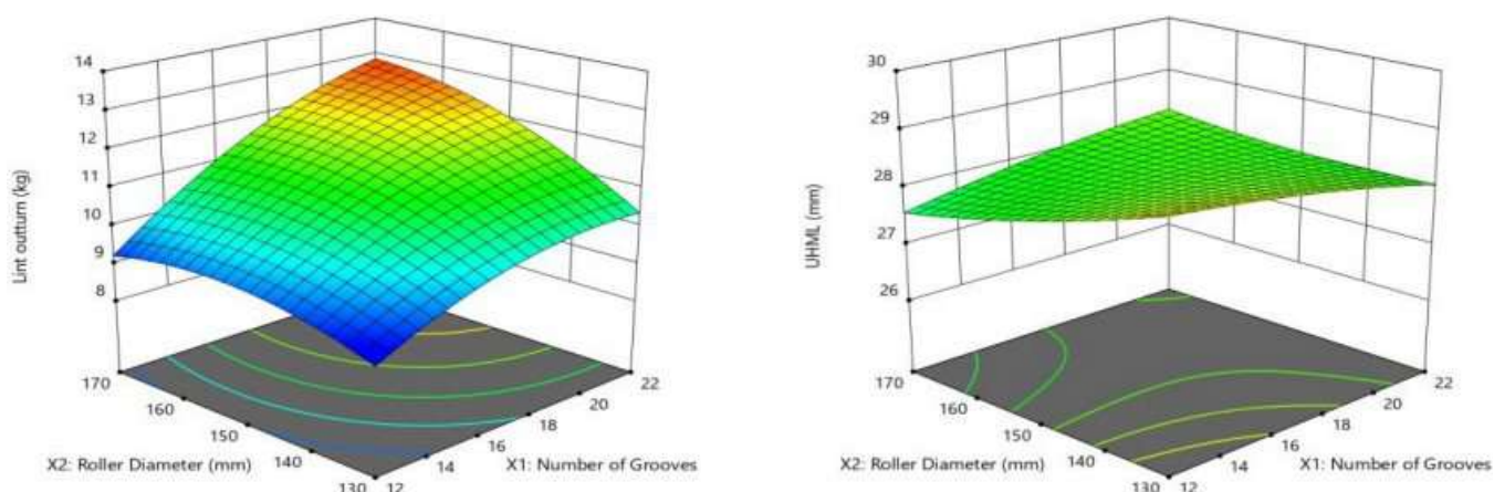
Fig 2.1. Effect of independent variables on a) lint outturn and b) UHML
