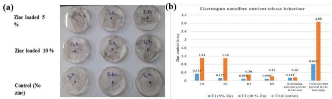
Fig:2.6 a. Electrospun nanofibre mat Nutrient releasing analysis b. Releasing behavior of zinc from zinc loaded electrospun mat at different time intervals
