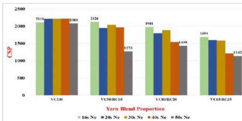
Fig 2.3. Effect of recycled fibre proportion and count on yarn CSP
