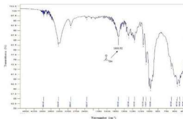
Fig. 2.34 FTIR analysis of TEMPO-oxidized cotton fibres
