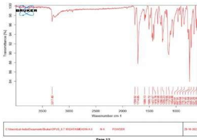
Pure Aceclofenac
